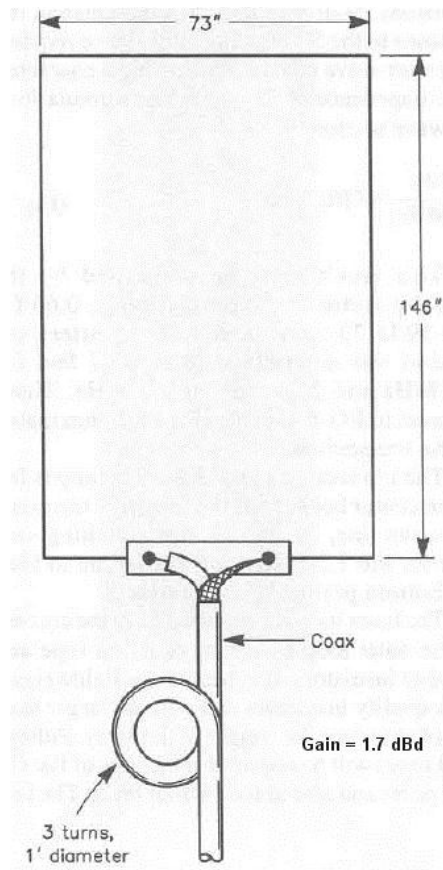
Lazy Quad Antenna for 10m
